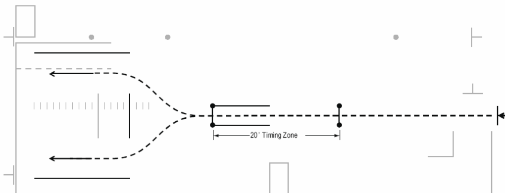
4. Obstacle swerve
